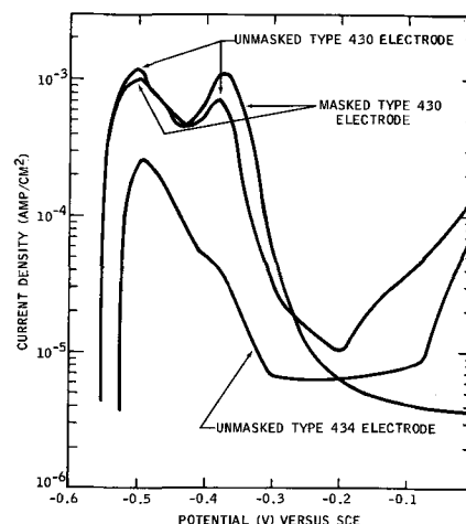
Fig. 1. Anodic potentiodynamic polarization curves for unmasked Types 430 and 434 electrodes and for masked Type 430 electrode in 0.1N hydrochloric acid at 29.6°C.
